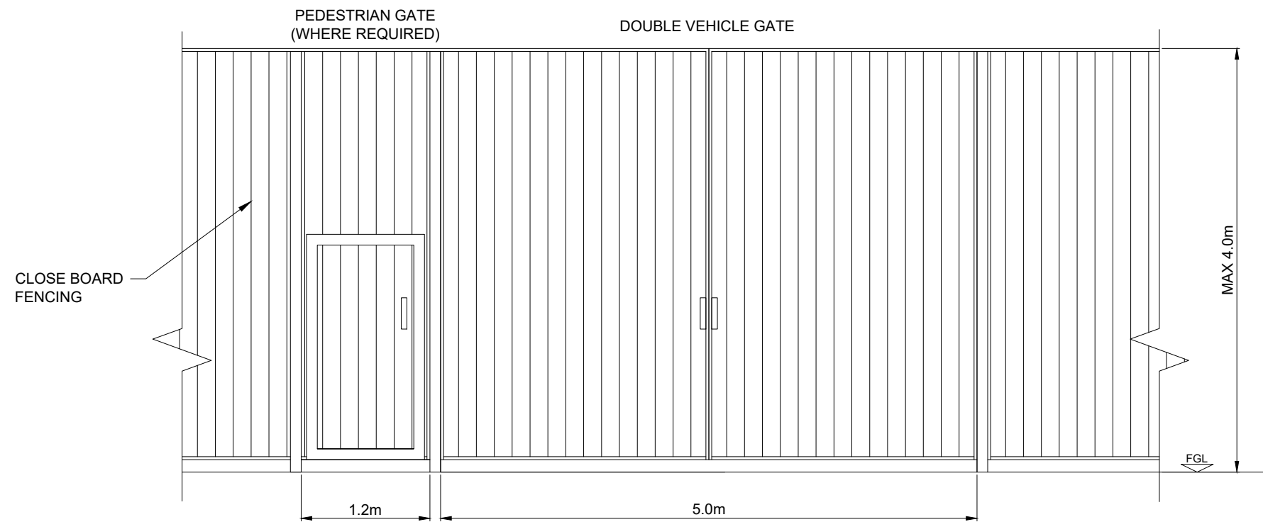
TYPICAL ELEVATION
